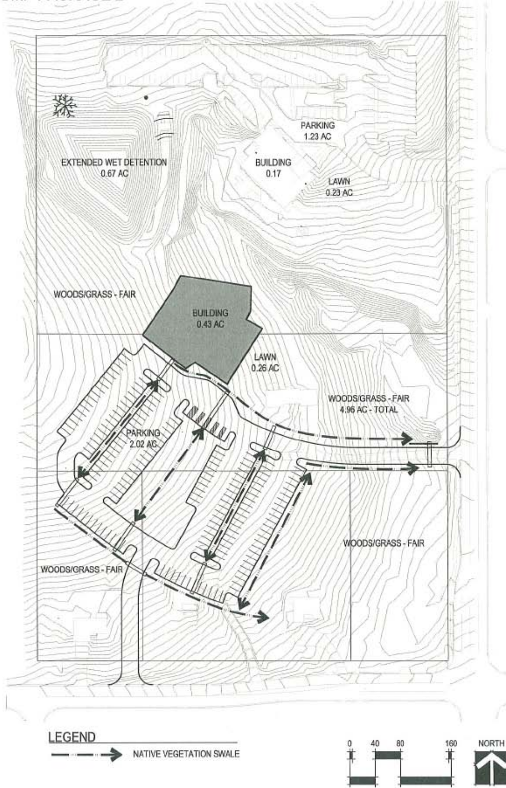
Figure 15: Example 3 BMP Package 2
